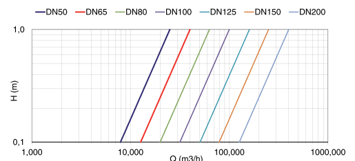
Head loss
